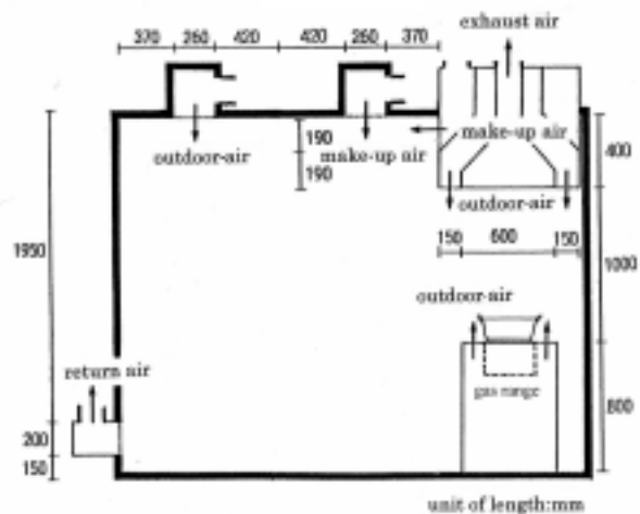
(2) Section
