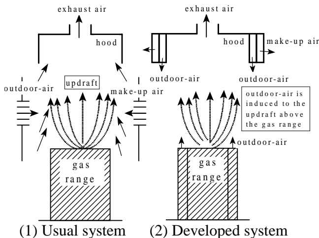
Figure 1 Outline of developed ventilation system
