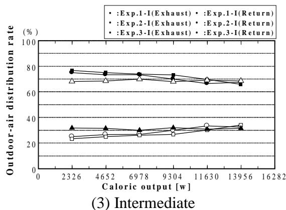
Figure 3 Outdoor-air distribution rate
