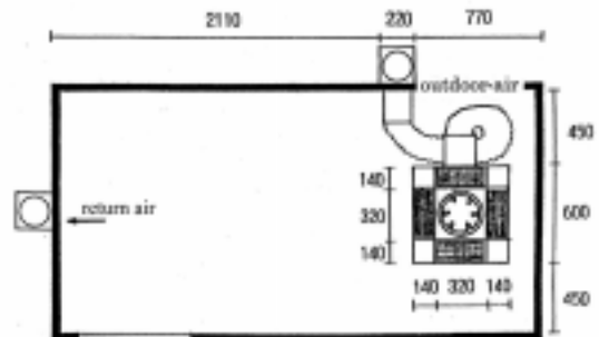
(1) Plan
