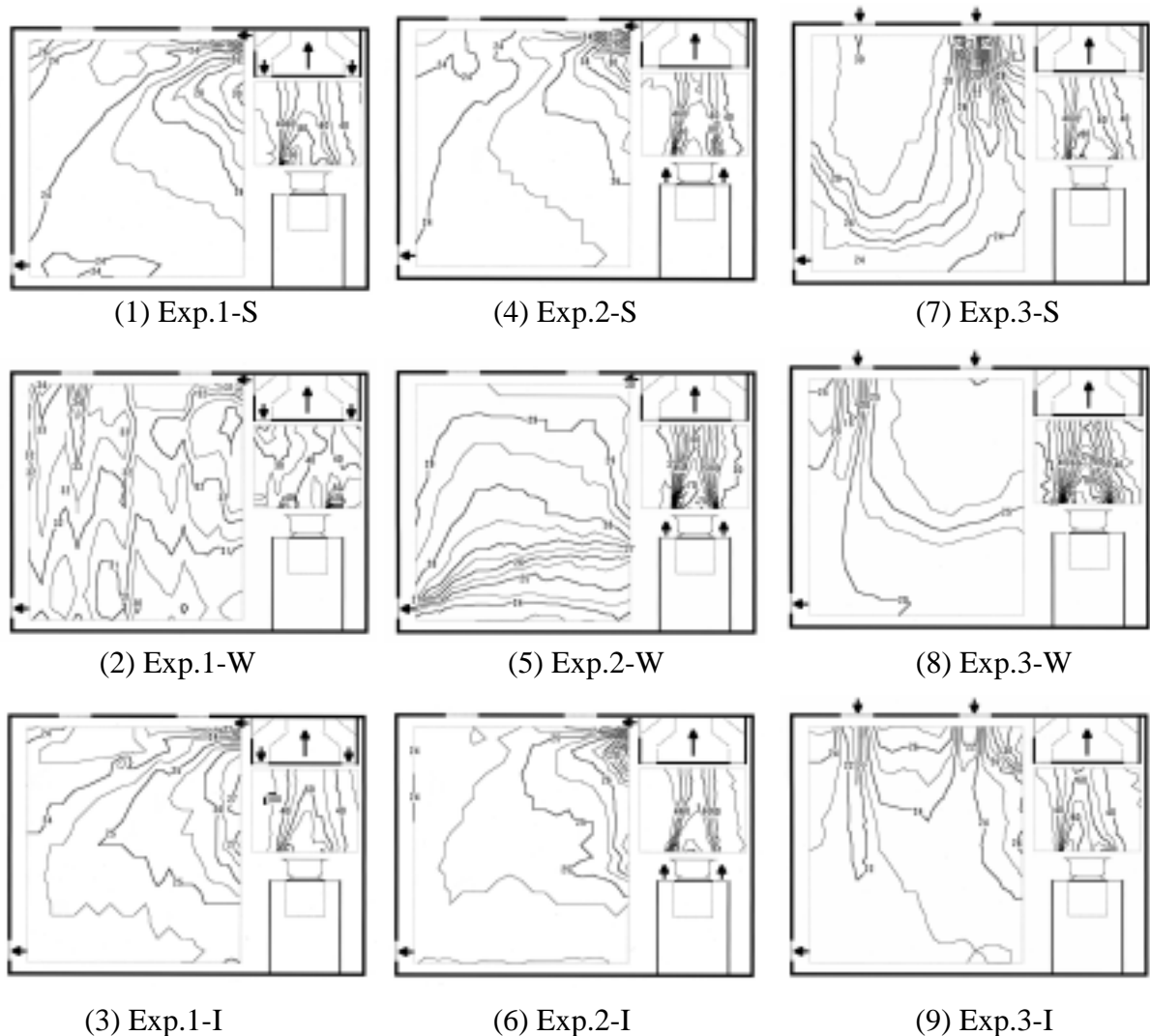
Figure 5 Temperature Distribution
