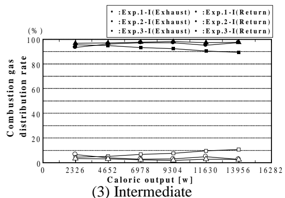
Figure 4 Combustion gas distribution rate
