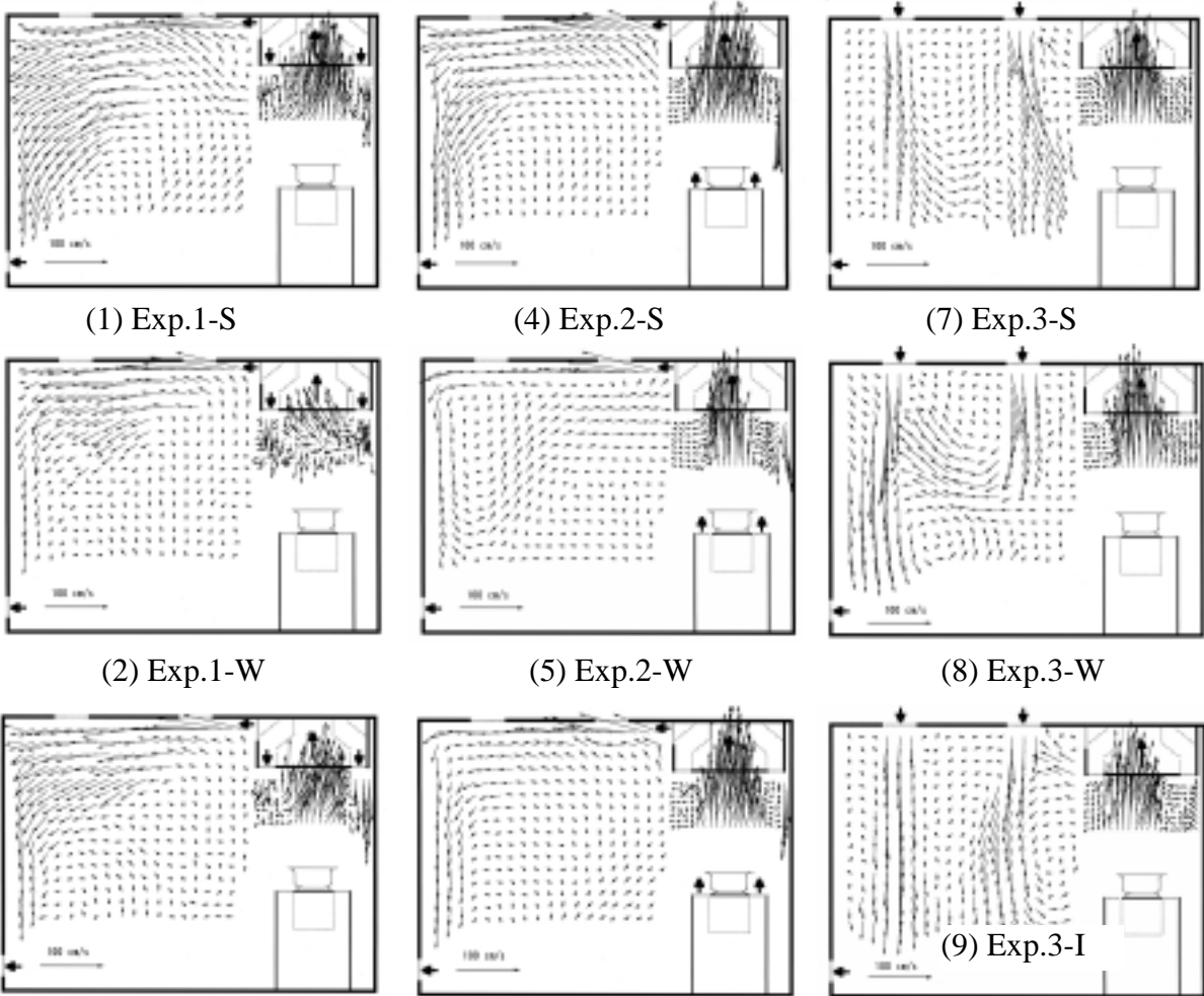
Figure 6 Air-flow distribution
