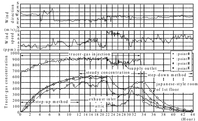
Figure 10 Concentration profile of Exp.B-2
