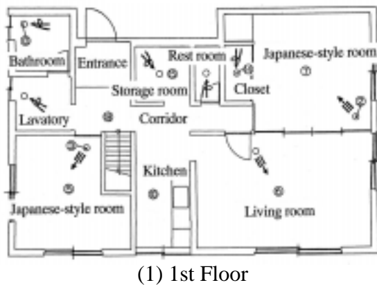
Figure 1 Floor plan of House A
