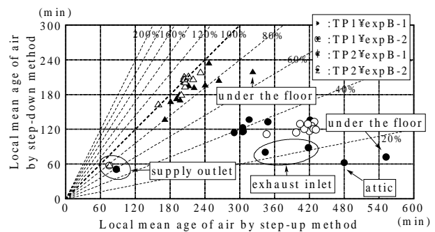
Figure 11 Local mean age of air of House B
