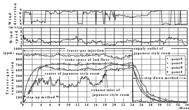
Figure 6 Concentration profile of House A
