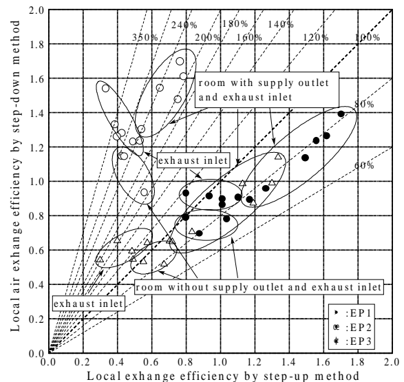
Figure 8 Air exchange efficiency of House A
