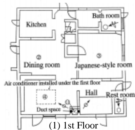
Figure 3 Floor plan of House B
