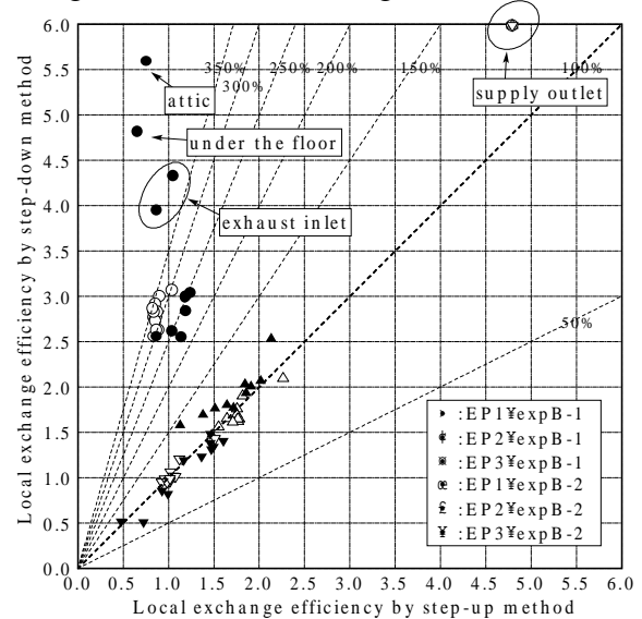
Figure 12 Air exchange efficiency of House B
