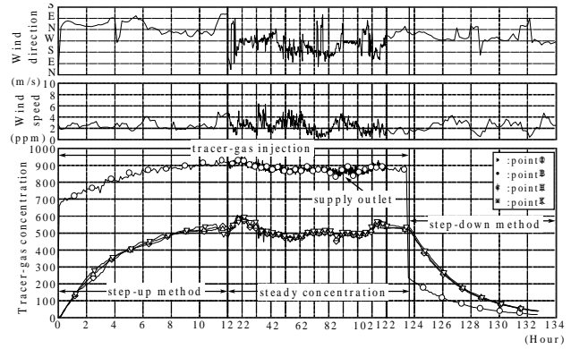
Figure 9 Concentration profile of Exp.B-1
