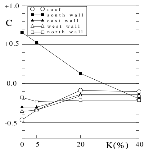
Figure 5. Variation of C with K (with flat roof)
