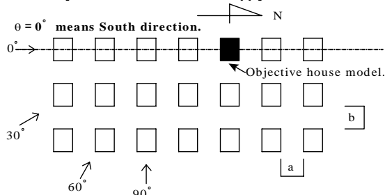
Figure 3. The arrangement of the house and a wind direction
