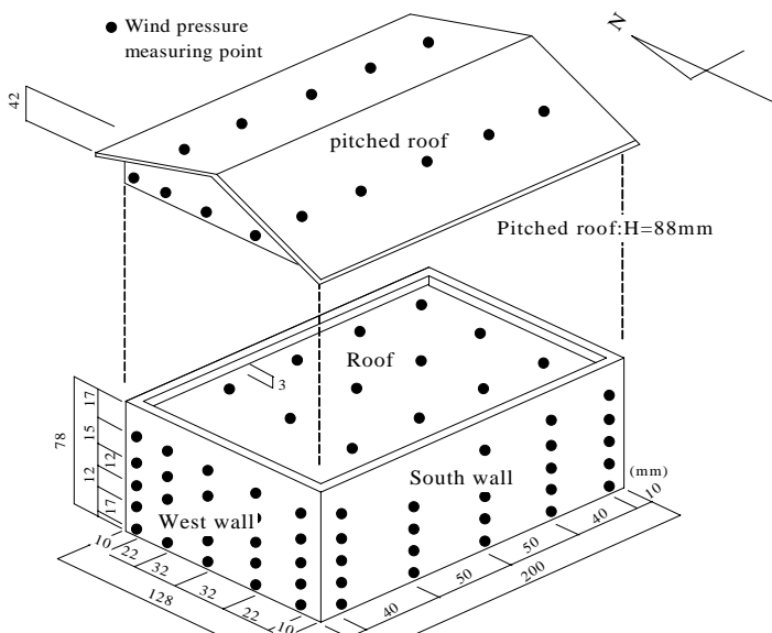
Figure 1. Model of the house and wind pressure measuring points
